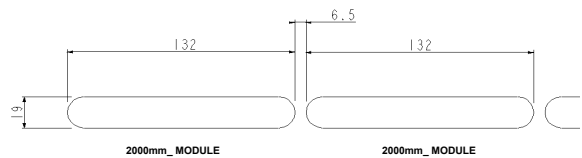
VENT ROUTING DETAIL 4000mm_ SHOWN BUT TYPICAL OF ALL SIZES
